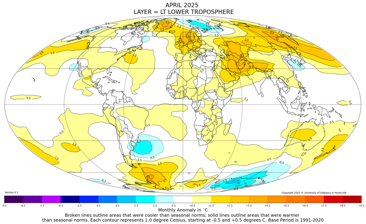
Figure. Lower tropospheric temperature anomalies for April 2025. Contour interval 1.0 °C.
