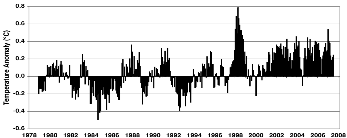
Fig. 1: Global variation from seasonal norms, in Celsius; Trend since Nov. 16, 1978: +0.14 C per decade
