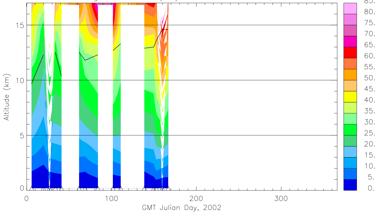
Integrated Ozone (DU) Over Old Huntsville, AL
