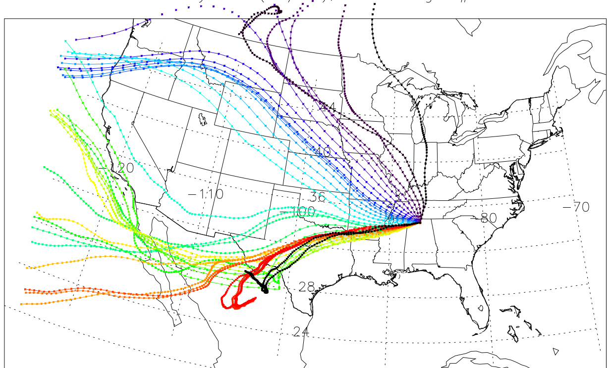
HYSPLIT 120-hour "Omega" Back-Trajectories (0–19.5 km) from Huntsville, AL 1800 GMT Day 138 (05/18), 2002 Flight #HU135
