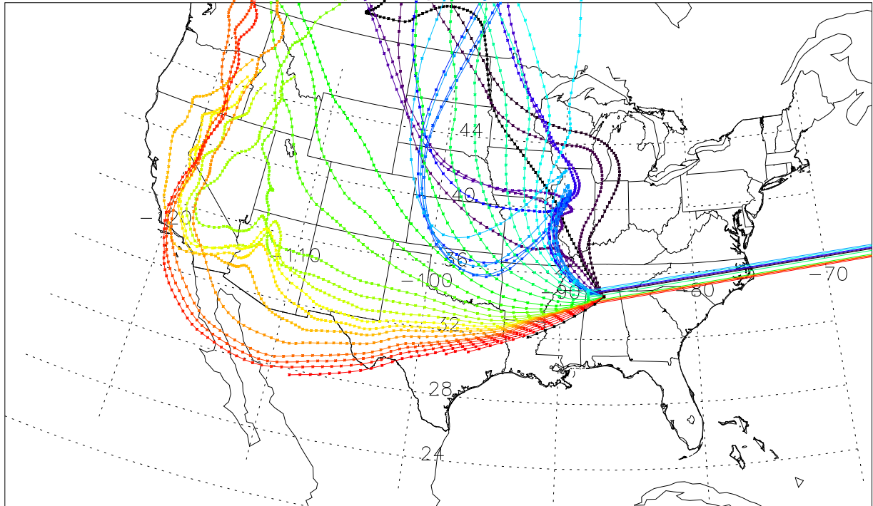
HYSPLIT 120-hour "Omega" Back-Trajectories (0–19.5 km) from Huntsville, AL 1800 GMT Day 020 (01/20), 2001 Flight #HU085
