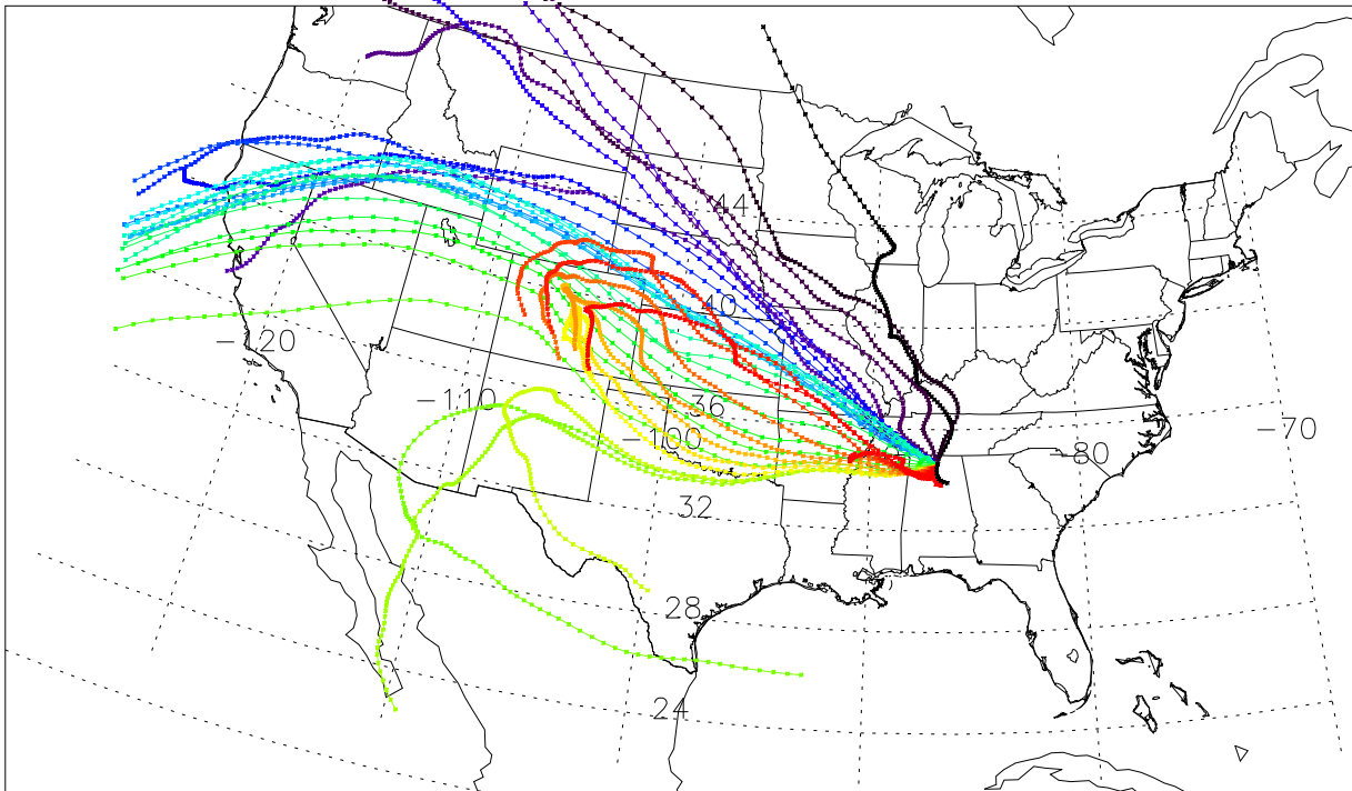
HYSPLIT 120-hour "Omega" Back-Trajectories (0–19.5 km) from Huntsville, AL 1800 GMT Day 204 (07/22), 2000 Flight #HU062
