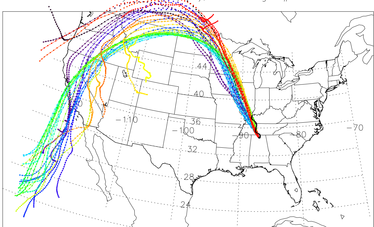
HYSPLIT 120-hour "Omega" Back-Trajectories (0–19.5 km) from Huntsville, AL 1900 GMT Day 197 (07/15), 2000 Flight #HU061
