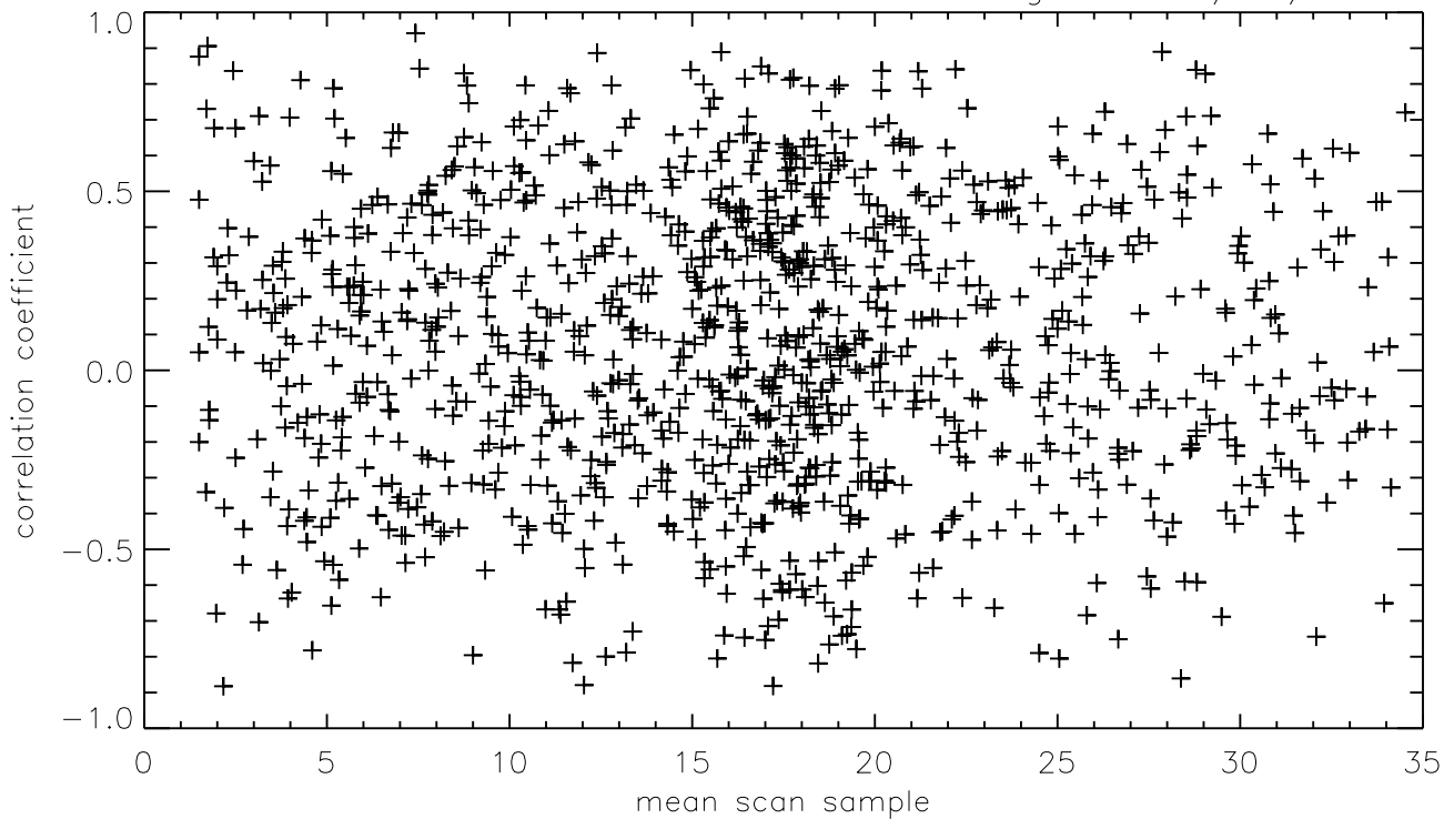
corr. coeff. vs. solar zenith and scan angle on 01/01/80
