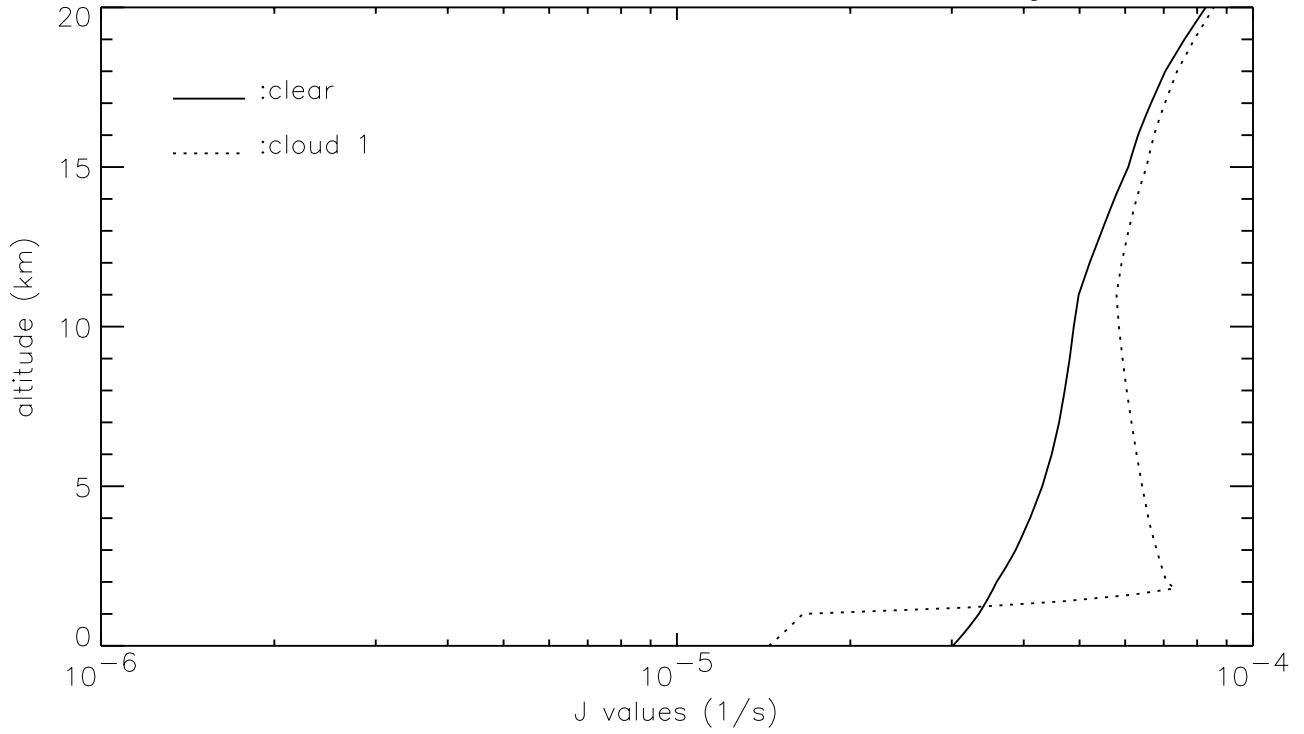
J-values vs. altitude: \text{sza}=0 , \text{O.D.}=20 , w=1 , g=0.85
