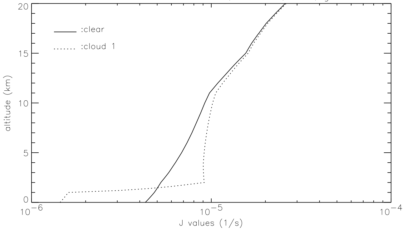
J-values vs. altitude: \text{sza}=60 , \text{O.D.}=20 , w=1 , g=0.85
