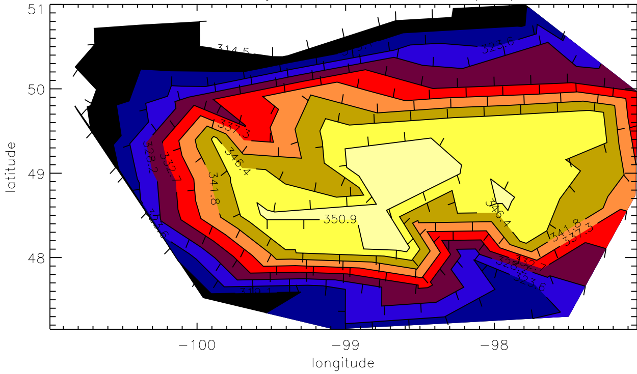
ozone anomaly in North Dakota on 6/29/89
