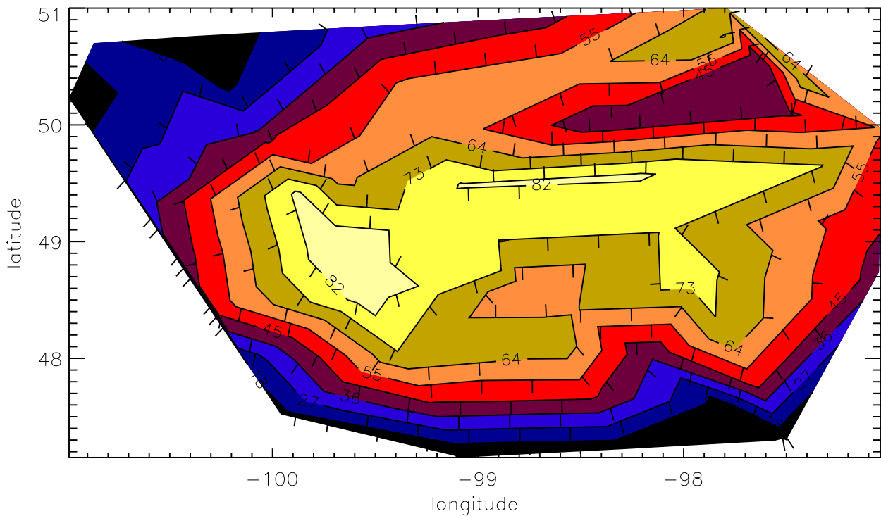
1. ozone contour 2. reflectivity contour
